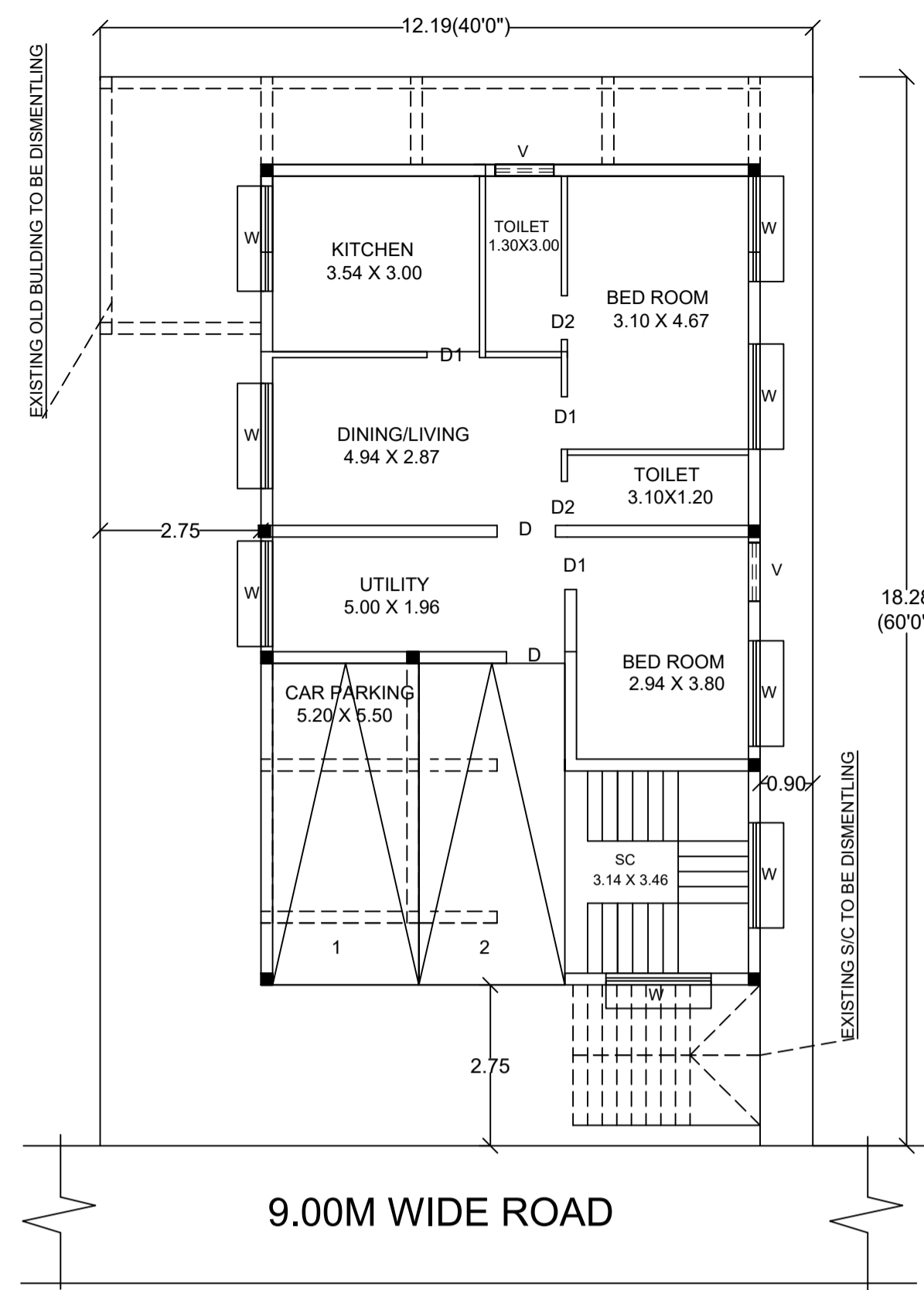
EXISTING GROUND & ADDITIONS FLOOR PLAN
