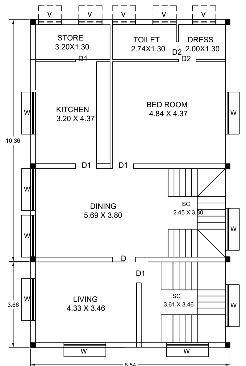
EXISTING FIRST FLOOR & ADDITIONS PLAN
